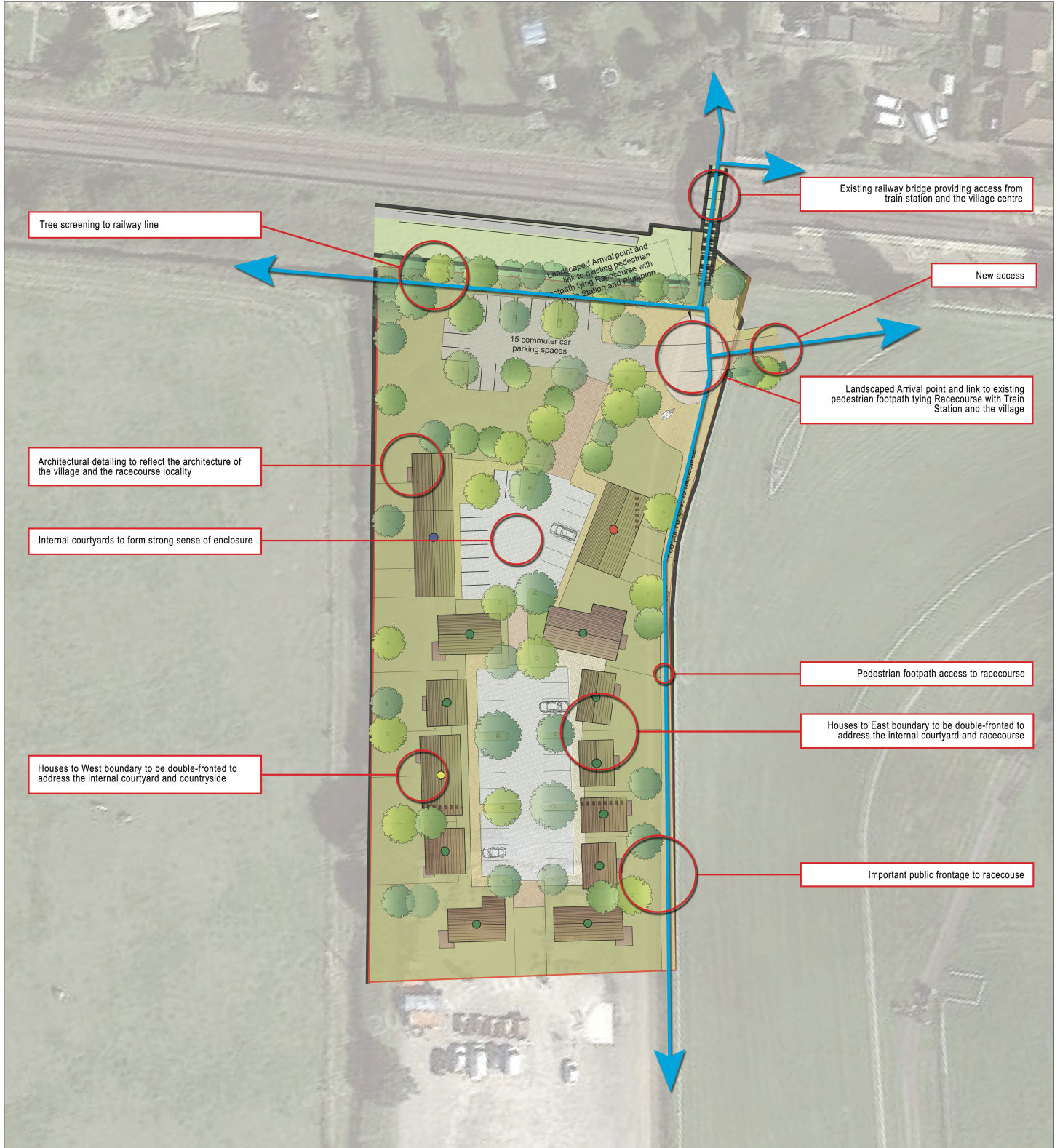
PROPOSED SITE PLAN - ILLUSTRATIVE LAYOUT
